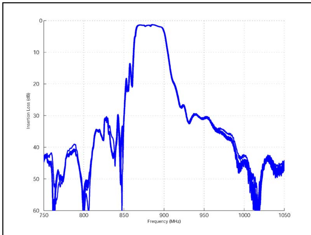
Typical measured response (S12)
